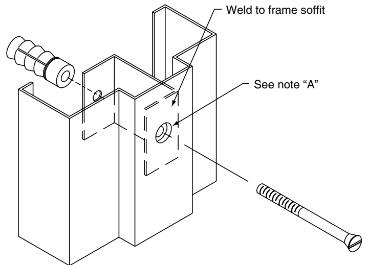
"C" Anchor
